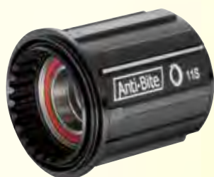
Shimano 11s Aluminum 7075 R10T-CBB1 69g ± 5g
